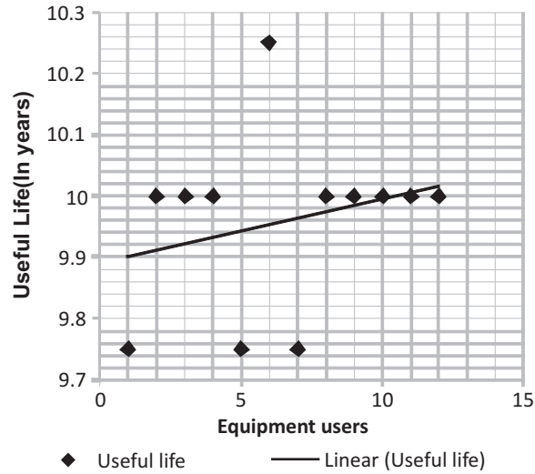
Figure 7. Useful Life of Hydraulic Pipe Bending Machine
